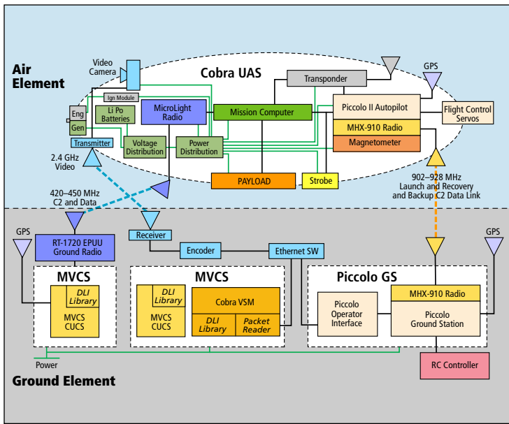
Cobra UAS block diagram
