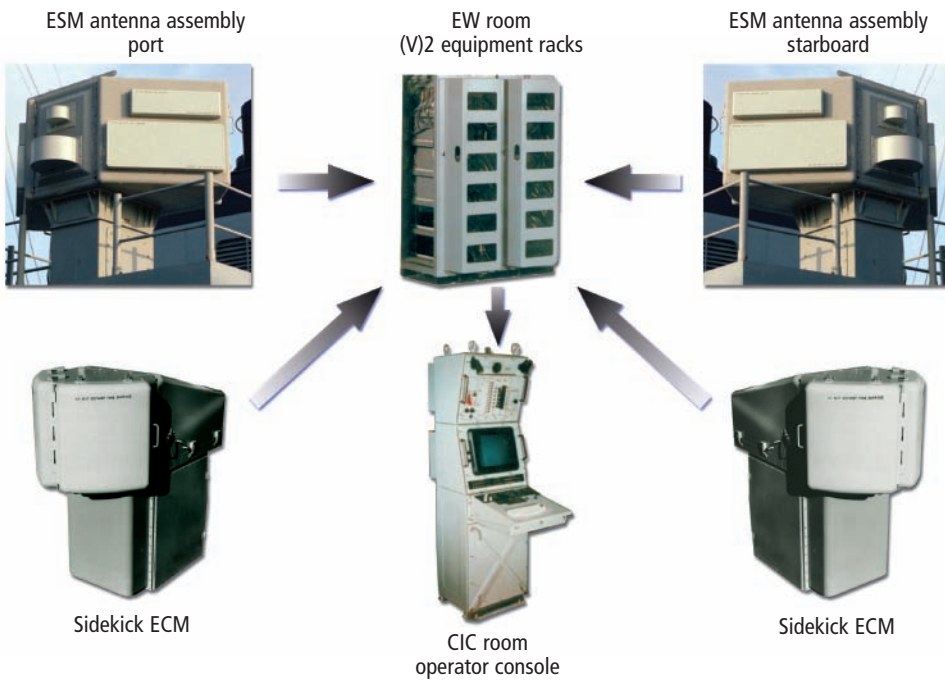
The AN/SLQ-32(V)5 features separate ECM and ESM enclosures above deck for flexible, cost-effective installation.
